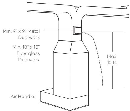
Installation Clearance
