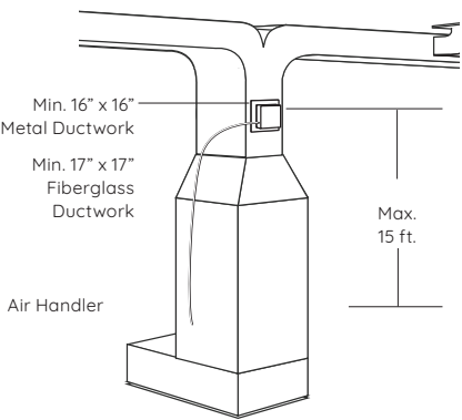
Installation Clearance
